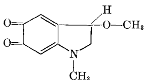
Adrenochrome methyl ether
