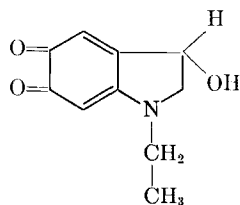
N -Ethylnoradrenochrome
