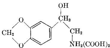
3,4-Methylenedioxy- \alpha - aminomethylbenzyl alcohol oxalate
