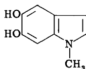
5,6-Dihydroxy- N -methylindole
