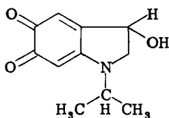
N -Isopropylnor-adrenochrome
