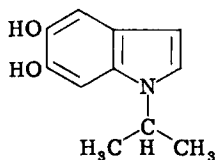
5,6-Dihydroxy- N -isopropylindole
